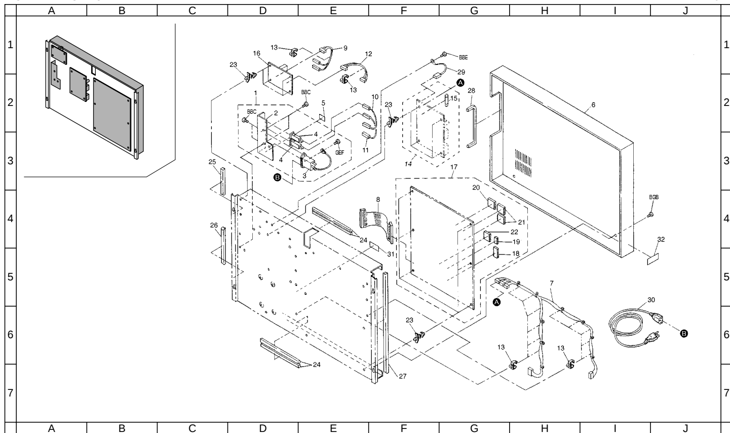
FIG. 1 MEMORY UNIT
